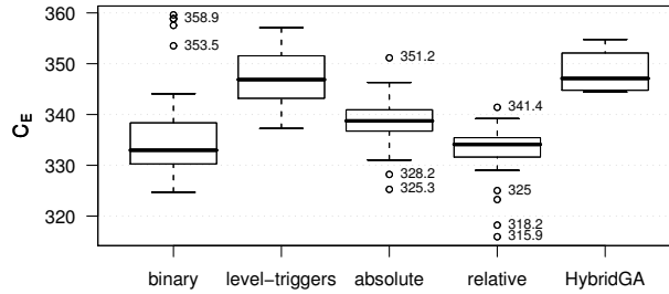
Figure 20: Boxplot of the results of SEA for different representations and Hybrid GA in the Vanzyl network.
